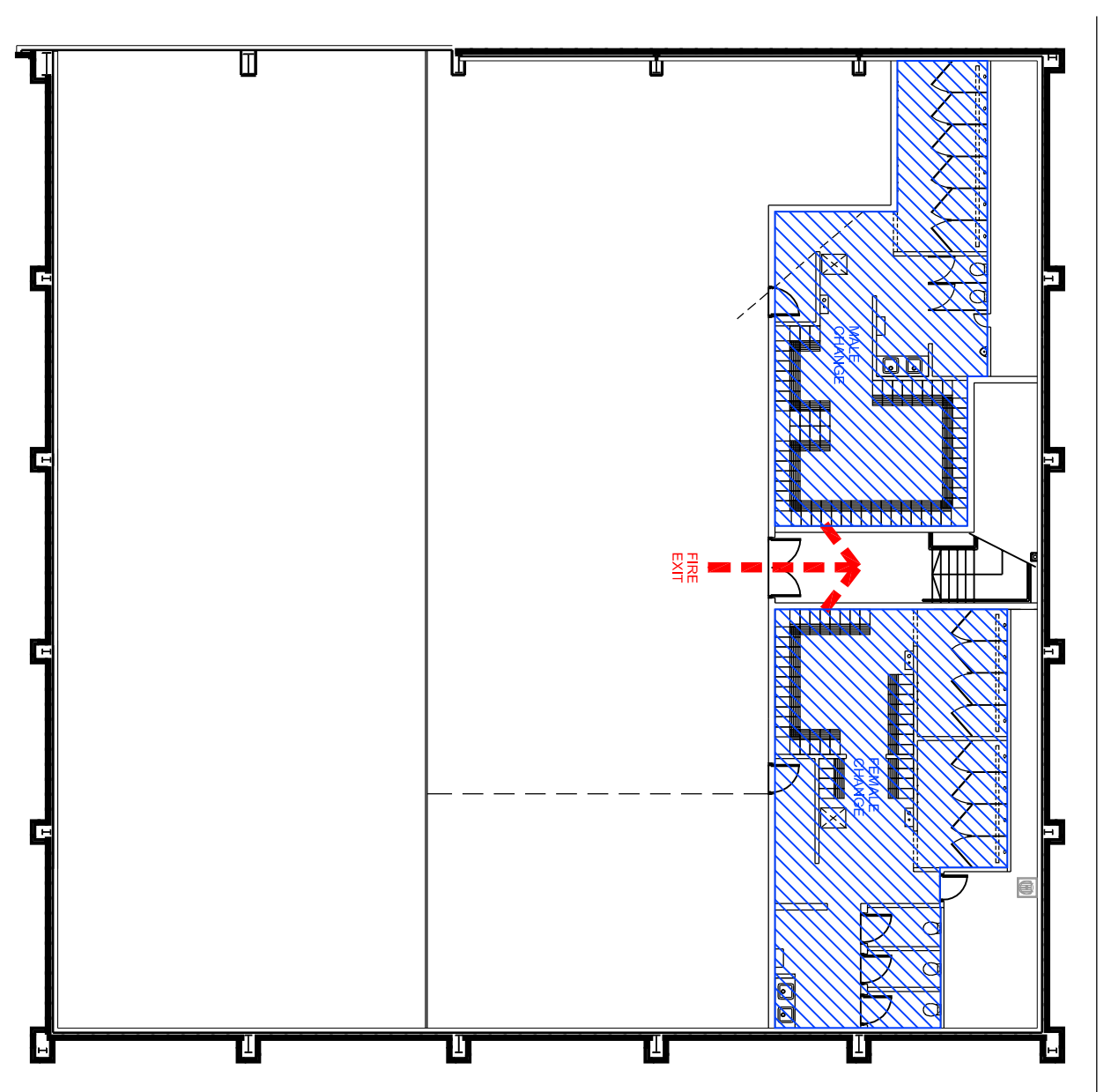
MEZZANINE FLOOR
